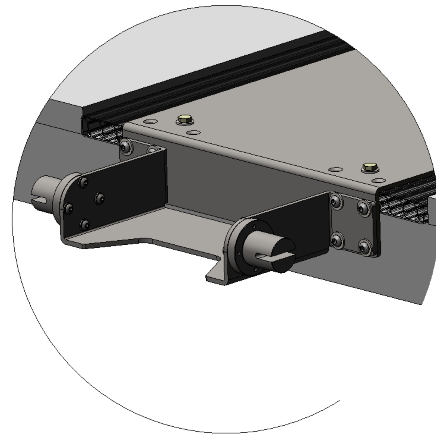
DETAIL B VINYL REMOVED
